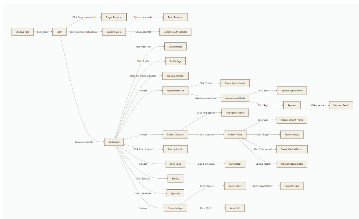
Figure 13. Screen Flow of Receptionist
