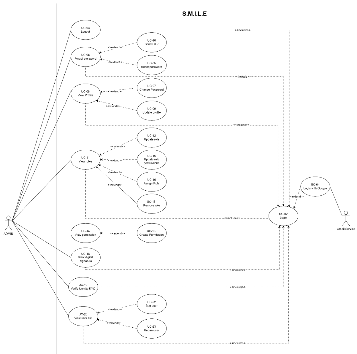
Figure 7. Use case diagram of Admin (1)
