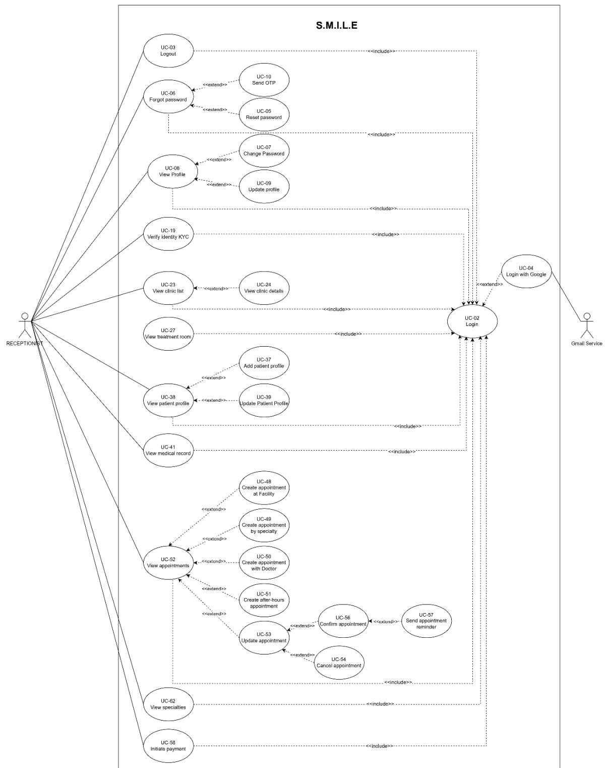
Figure 9. Use case diagram of Receptionist
