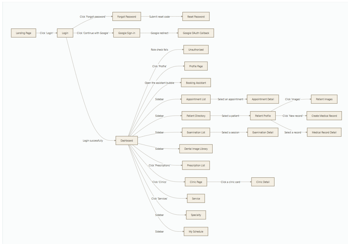
Figure 12. Screen Flow of Nurse
