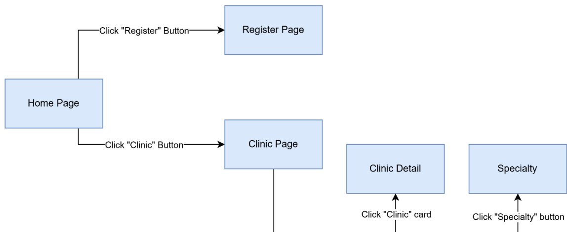
Figure 15. Screen Flow of Guest
