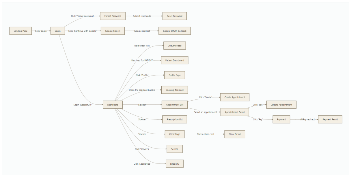
Figure 14. Screen Flow of Patient
