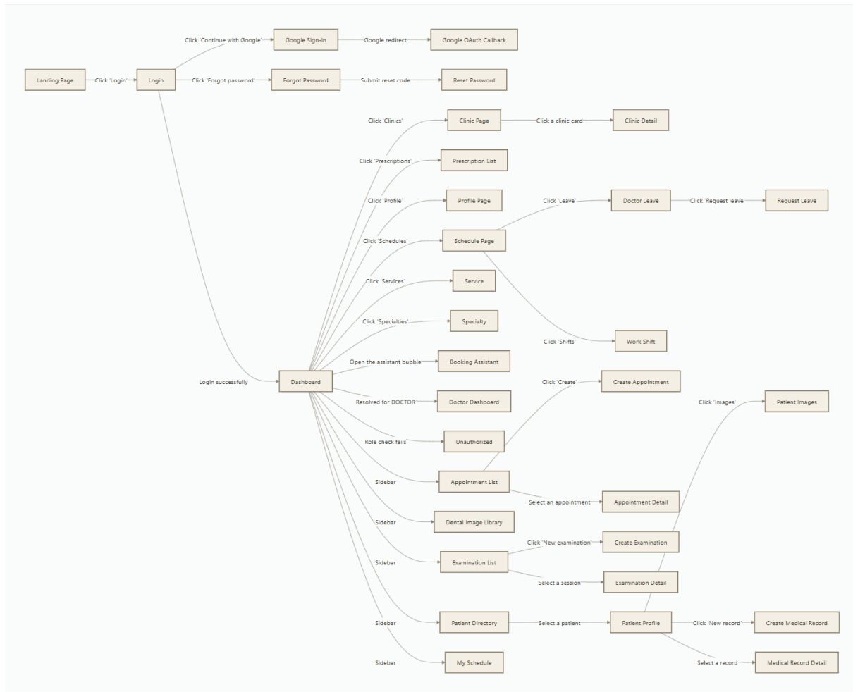
Figure 11. Screen Flow of Doctor
